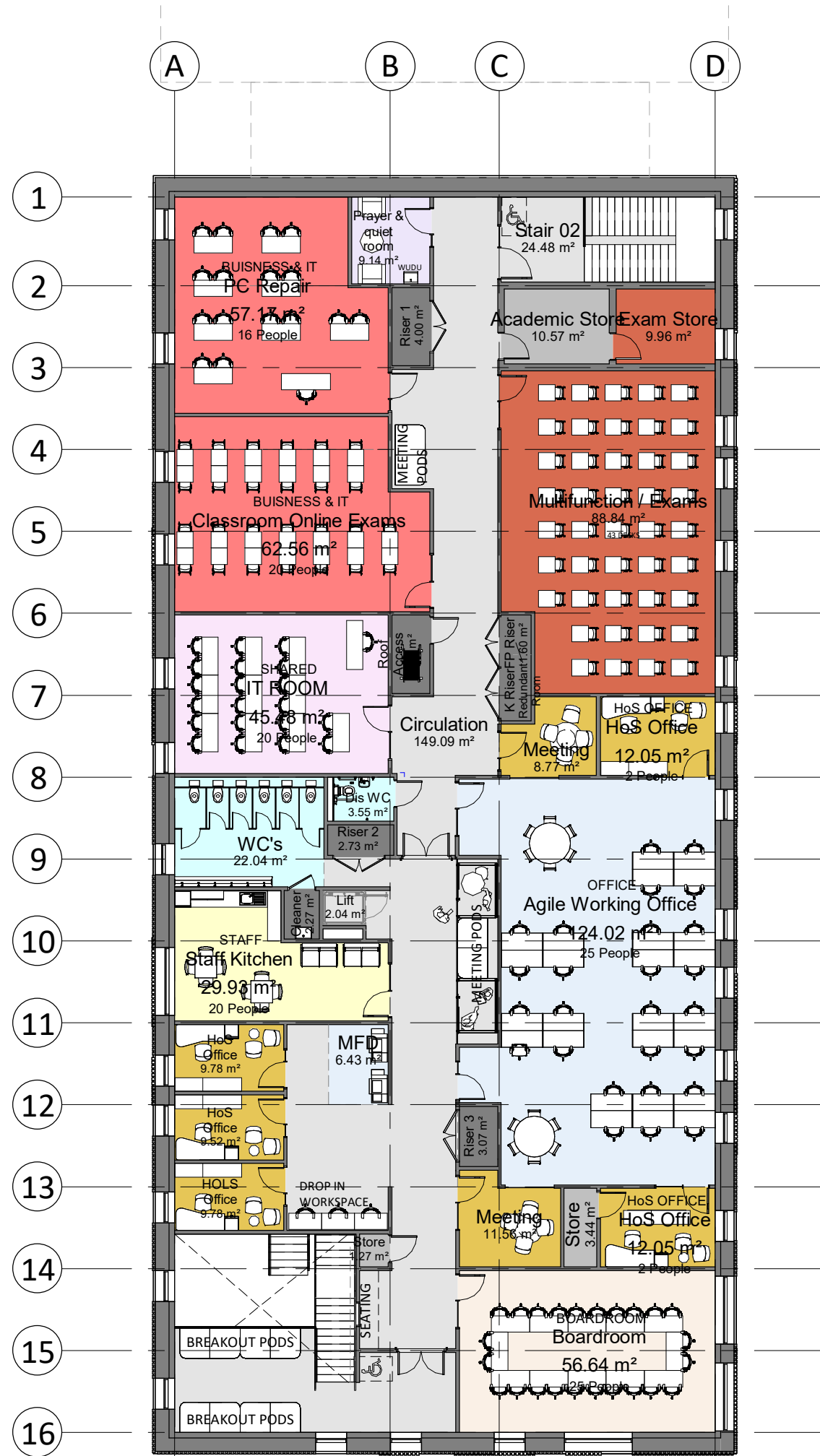
Proposed 02 Second Floor Plan 1 : 200
