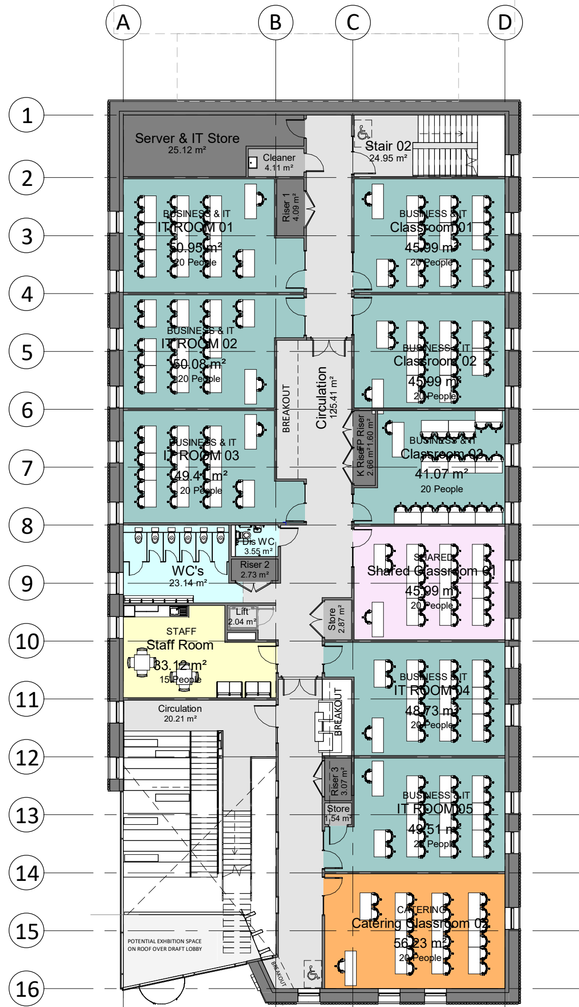
Proposed 01 First Floor Plan 1 : 200
