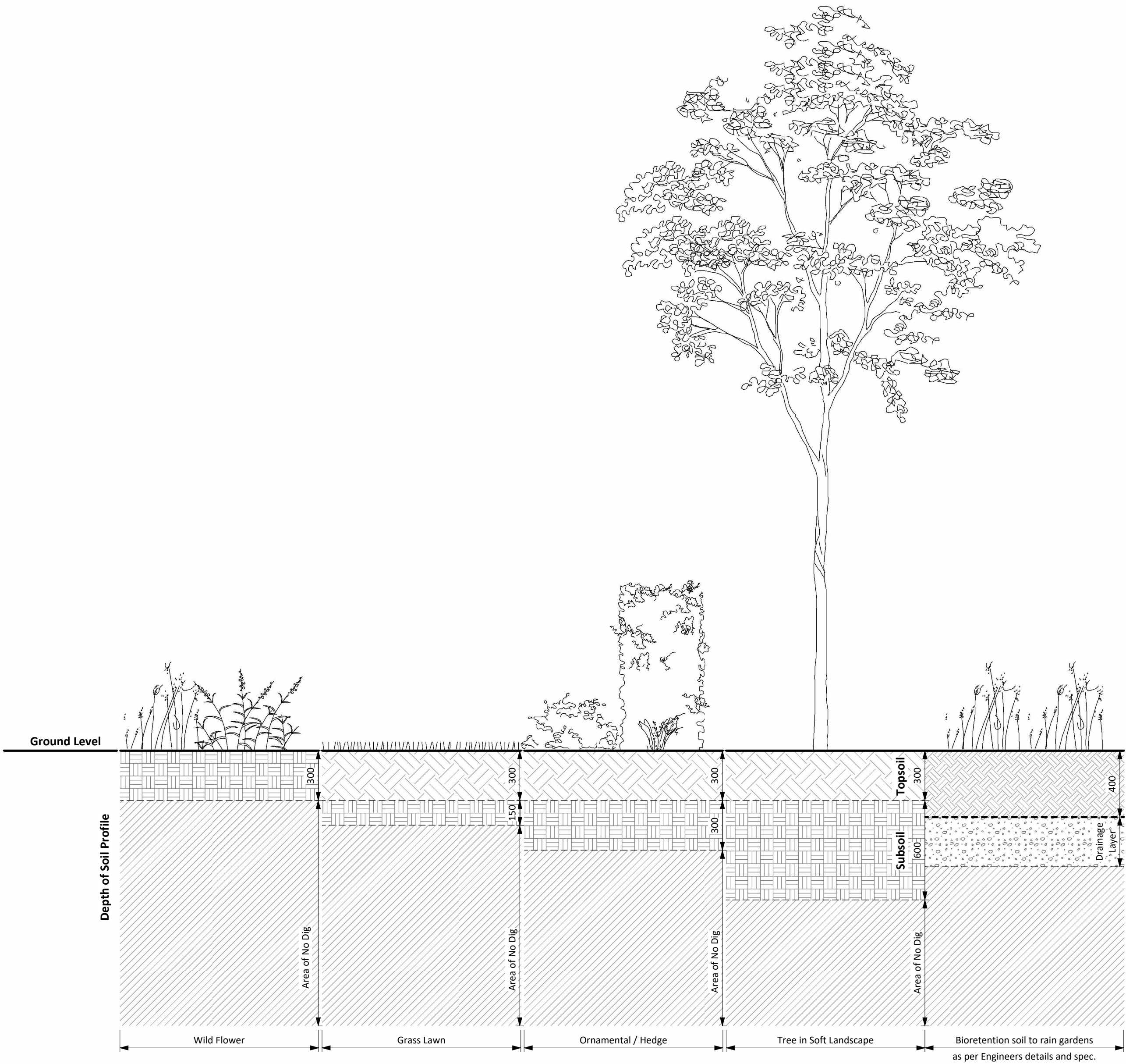
TYPICAL SOIL PROFILES FOR SOFT LANDSCAPE - BS 3882:2015
